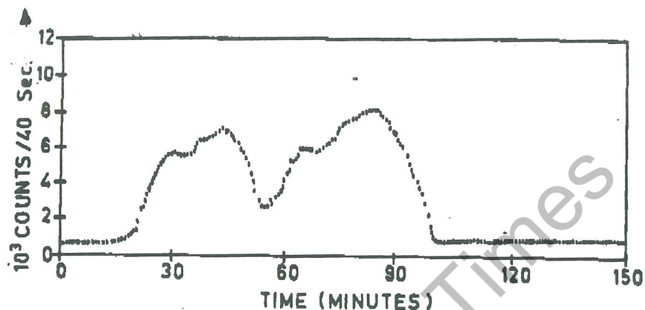
Fig.2. Neutron-Yield Variation During Description Mode: D 2 O Gas Loaded Titanium-Experiments (7 th June 1989)
