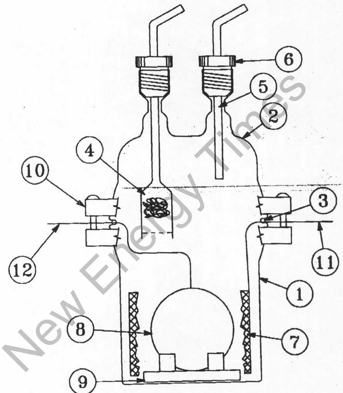
Figure C2 Electrochemical Cell
