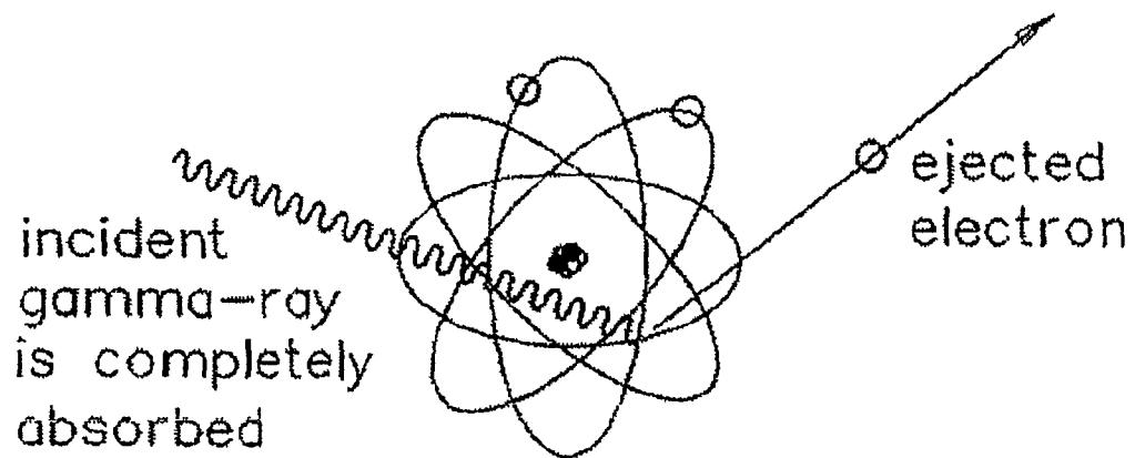
Figure 3. Photoelectric Effect – primarily low energy photons with E \leq 0.5 \text{ MeV}
