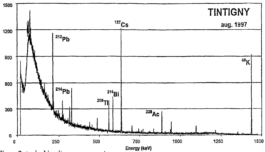
Figure 2: typical in-situ gamma-spectrum
