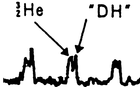
FIGURE 17.5 Arata shows the presence and separation of He-3 and HD in QMS.
