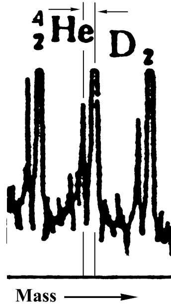
FIGURE 16.3 Arata shows the presence as well as the separation of He-4 and D 2 in a quadrupole mass spectrometer (QMS).
