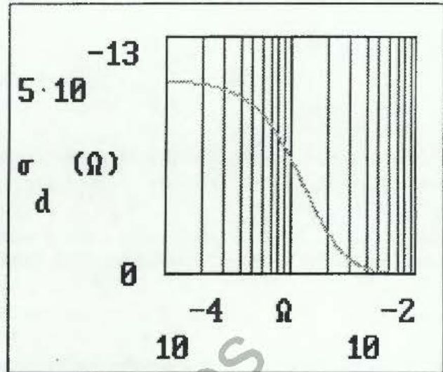
Figure 4: Deuterium Cross Section per unit solid angle.
