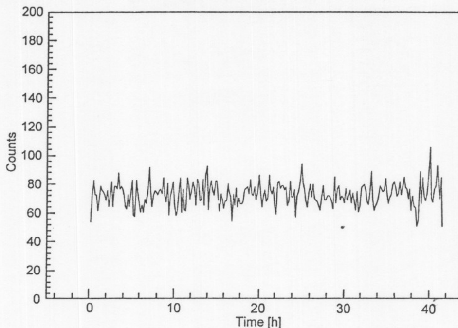
Fig. 4. - Counting rate of detector C2 placed 39 cm away from the cell (42 hours in the period 19-26 June 1995). Each point represents the number of pulses recorded in 10 minutes.
