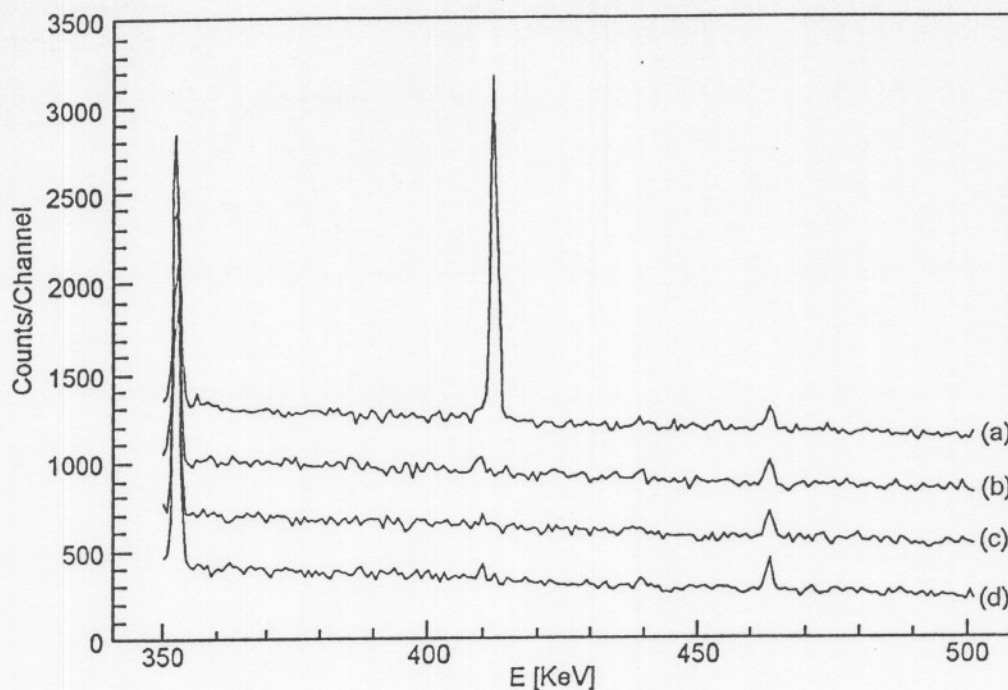
Fig. 5. - Gamma-ray spectra in the 350-500 keV region obtained with a germanium detector for: (a) gold sheet after the activation for 12 days on cell A; (b) gold sheet after the same exposition time to cosmic rays 10 m away from the cell; (c) gold sheet before the activation on the cell; (d) laboratory background.
