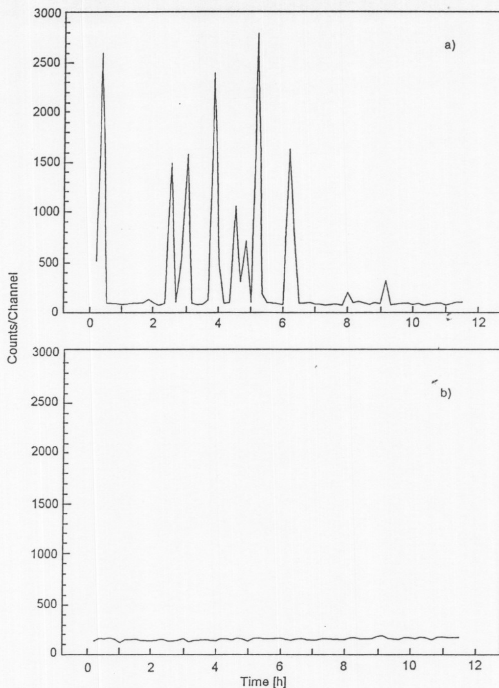
Fig. 2. - a) Counting rate of detector C2 placed 39 cm away from the cell (11 March 1995). Each point represents the number of pulses recorded in 10 minutes. b) Counting rate of detector C1 placed 10 m away from the cell (laboratory background). Each point represents the number of pulses recorded in 10 minutes.
