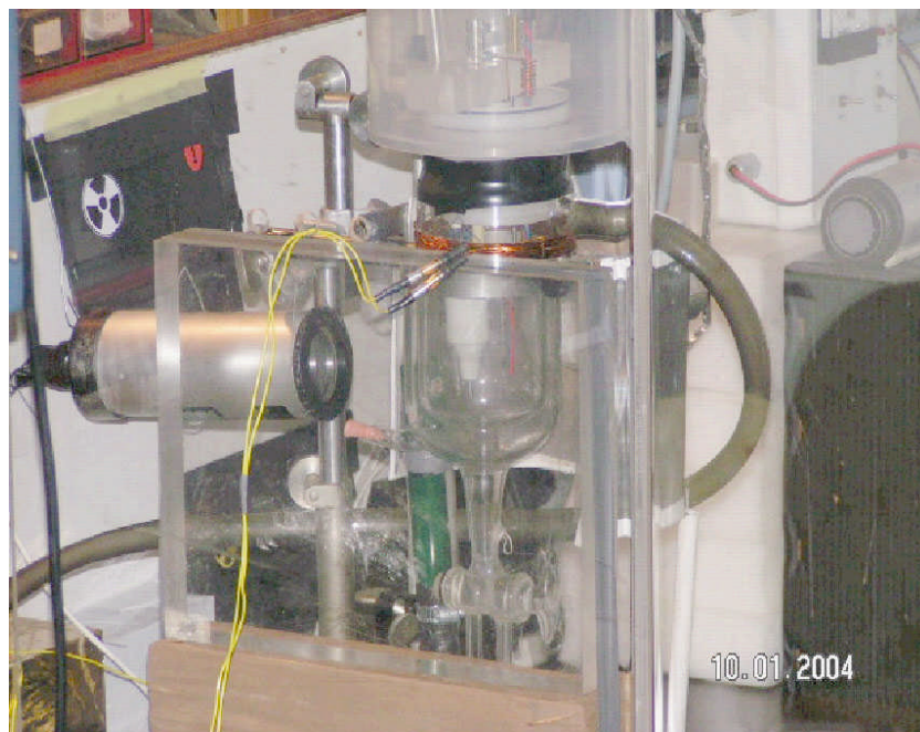
Fig. 3. Electrochemical Plasma Cell
