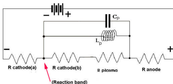
Fig. 17 Equivalent circuit of the cell during plasma phase
