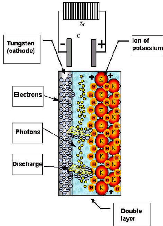
Fig. 6. Describing the Double layer during the ignition phase
