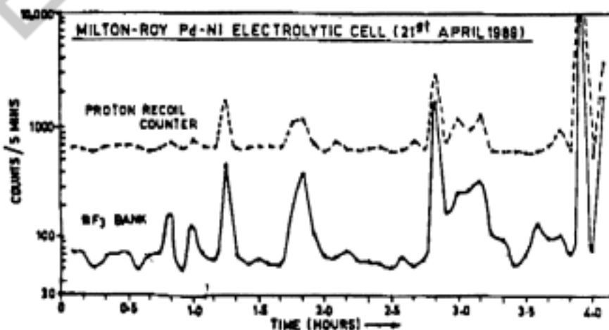
Fig.1. Neutron Counts Data From Two Detectors Using Milton-Roy Pd-Ni Electrolytic Cell (21 st April 1989)
