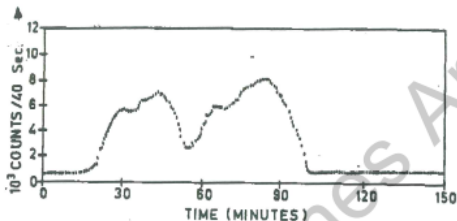
Fig.2. Neutron-Yield Variation During Desorption Mode: D 2 O Gas Loaded Titanium-Experiments (7 th June 1989)
