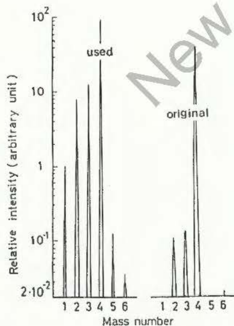
Fig. 5. Typical mass spectra of used gas in the reaction bulb and that of original deuterium gas.
