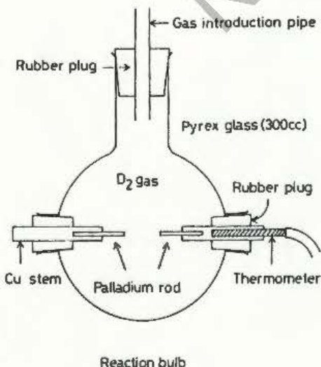
Fig. 1. Schematic diagram of the reaction bulb.
