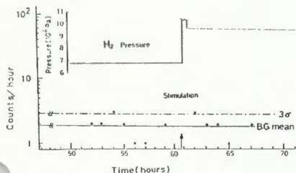
Fig. 4. Time dependence of neutron-detection for the experiment with hydrogen gas instead of deuterium. Stimulation is pointed by an arrow.
