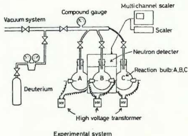
Fig. 2. Schematic diagram of the neutron measuring system.
