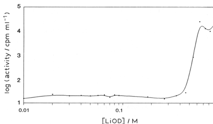
Fig. 1. The effect of electrolyte concentration on chemiluminescence of the scintillation cocktail.
