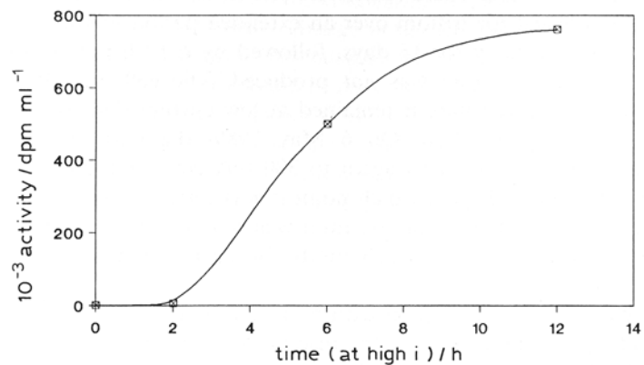
Fig. 3. The production of tritium in the electrolyte of cell A7 as a function of time.
