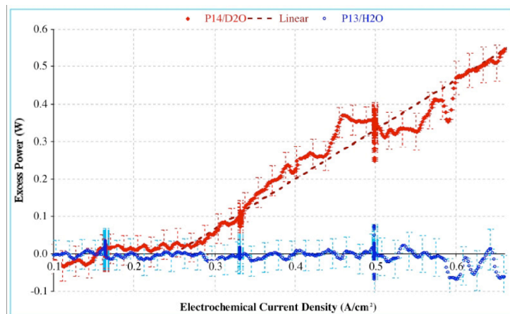
Figure 1: Graphs showing excess heat production versus current density in a cell similar to the Pons and Fleischmann one. In red a cell with D_2O , and in blue the same with H_2O
