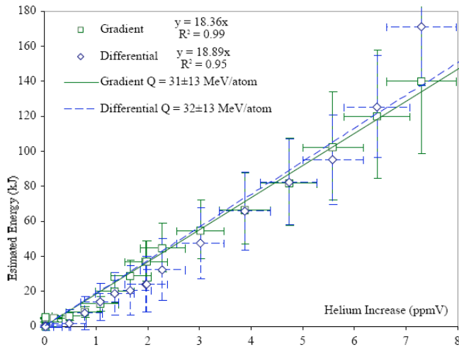
Figure 2: Heat production versus helium formation during an experiment.
