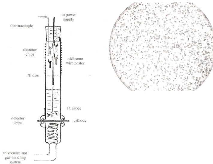
Figure 3: Left: electrochemical cell used by Oriani et al. [11] to detect alpha particles. Right: a micrograph showing large quantities of pits due to alpha particles.
